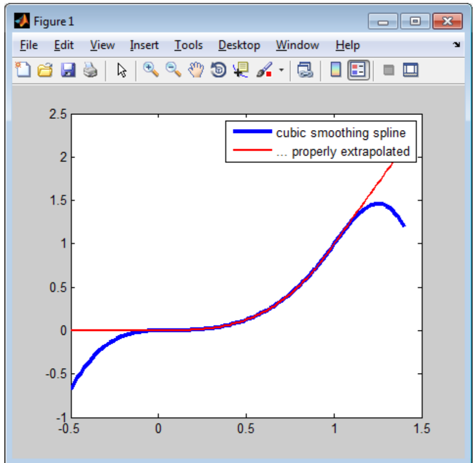
A Cubic Smoothing Spline Properly Extrapolated
